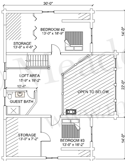
UPPER FLOOR PLAN 1,061 Sq. Ft.
