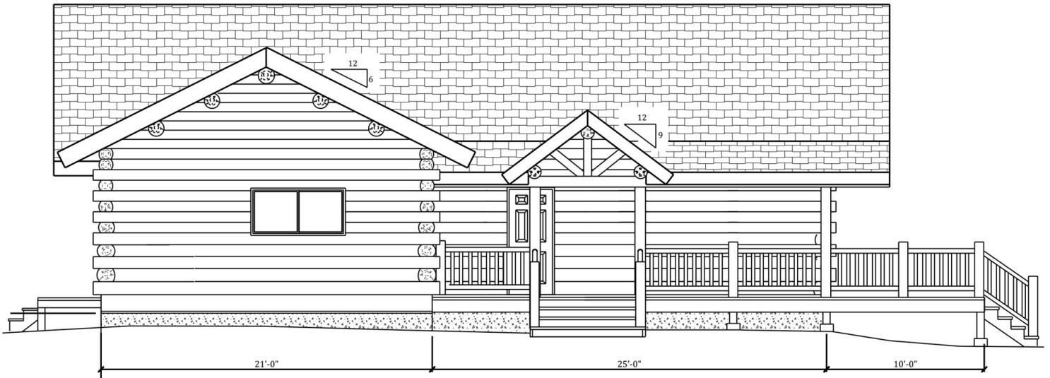
WEST ELEVATION
