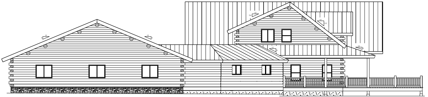
LEFT ELEVATION
