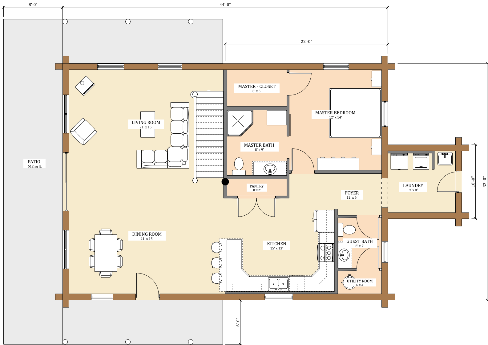
MAIN FLOOR
