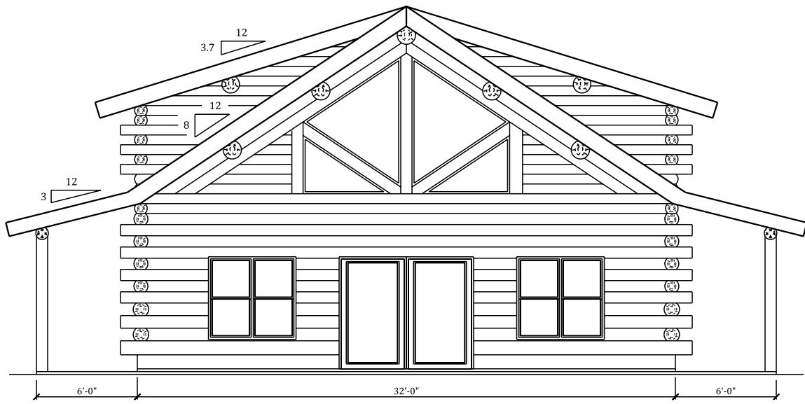
FRONT ELEVATION
