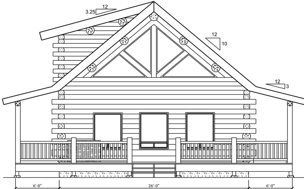
FRONT ELEVATION
