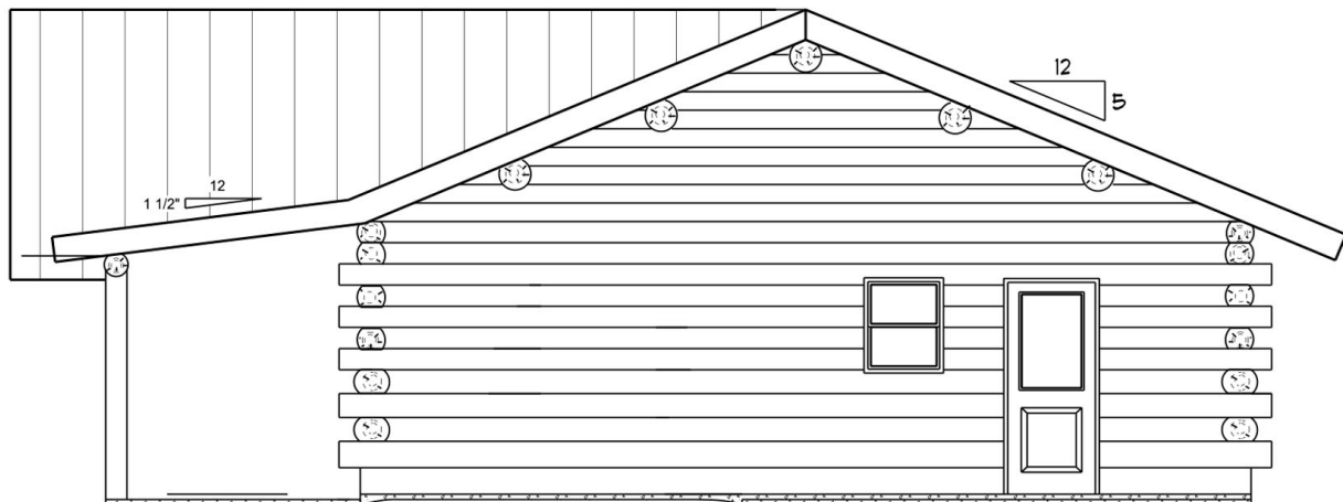
LEFT ELEVATION
