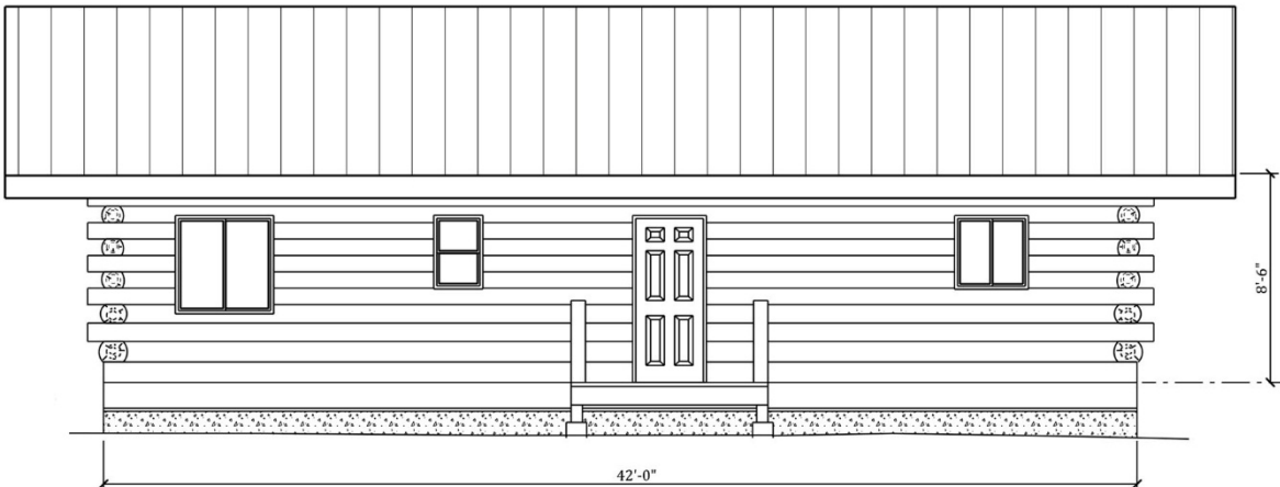
REAR ELEVATION
