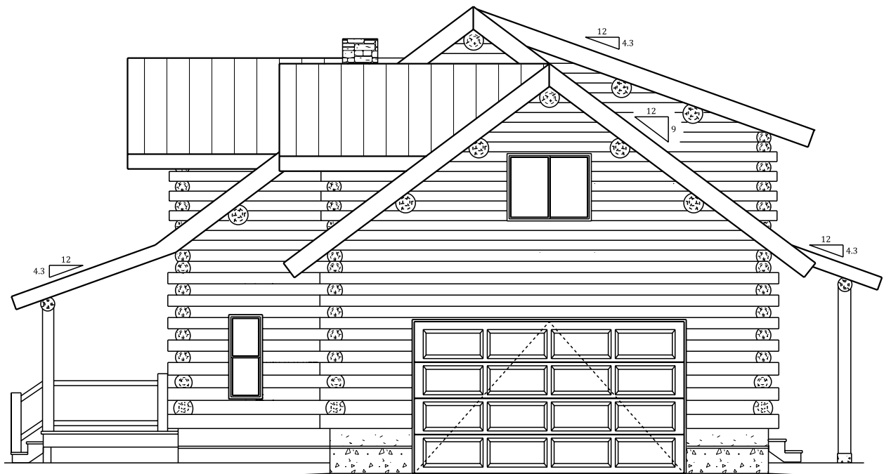
LEFT ELEVATION
