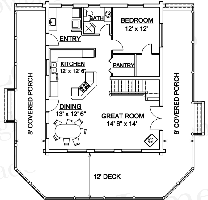
MAIN FLOOR 1140 Sq. Ft.
