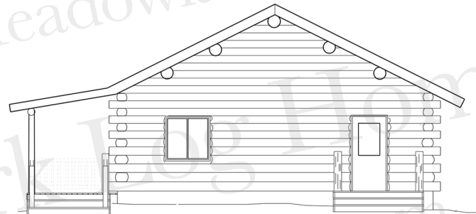
LEFT ELEVATION
