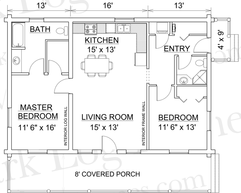
MAIN FLOOR 1,176 Sq. Ft.
