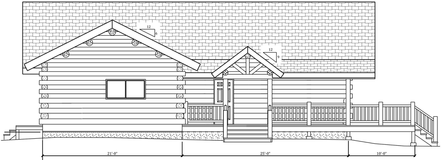
WEST ELEVATION
