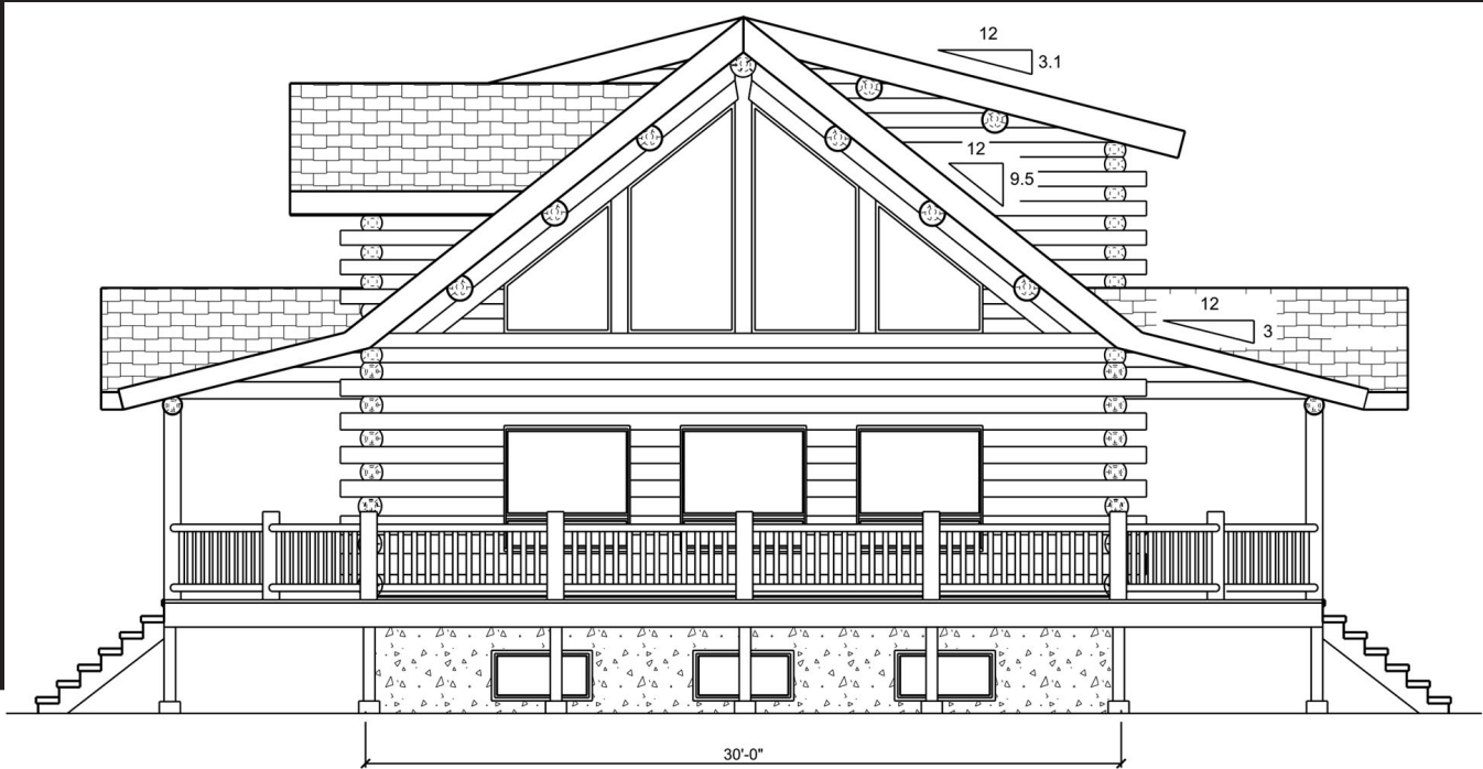
FRONT ELEVATION
