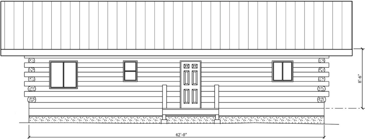
REAR ELEVATION
