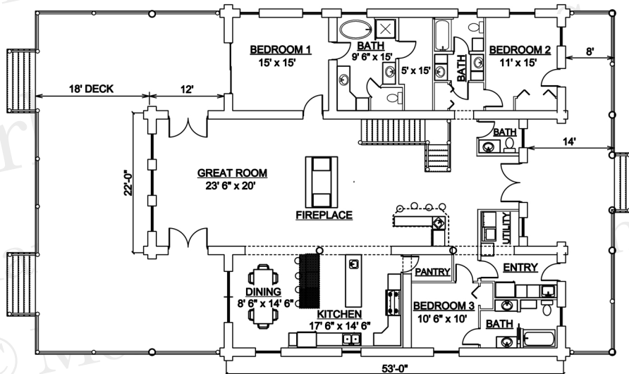
MAIN FLOOR 3007 Sq. Ft.
