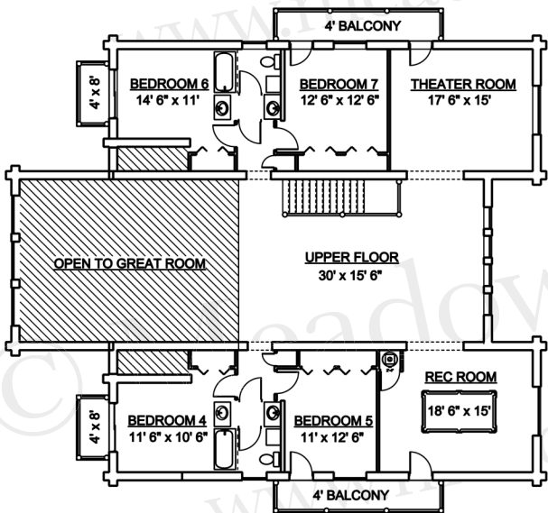
UPPER FLOOR 2271 Sq. Ft.
