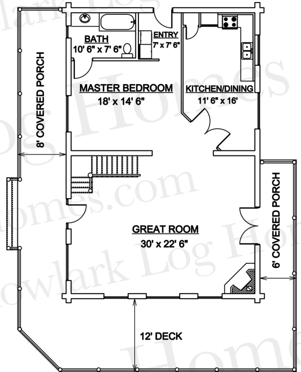
MAIN FLOOR 1536 Sq. Ft.
