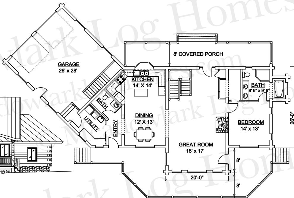
MAIN FLOOR 1715 Sq. Ft.
