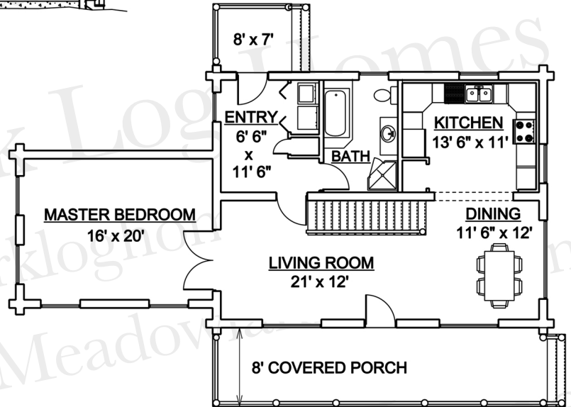
MAIN FLOOR 1204 Sq. Ft.
