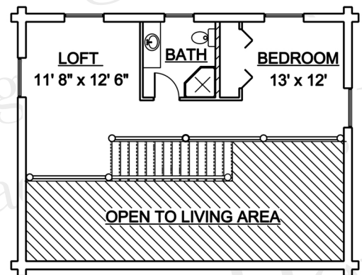
LOFT 472 Sq. Ft.
