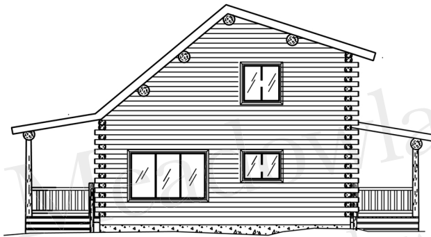
LEFT ELEVATION
