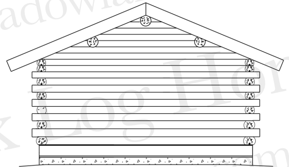
REAR ELEVATION
