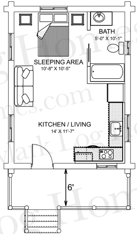
FLOOR PLAN
