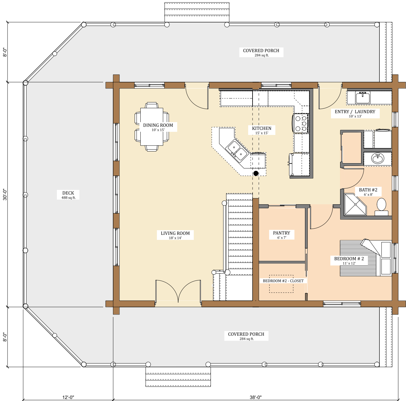
MAIN FLOOR
