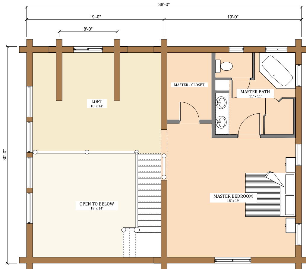
LOFT FLOOR
