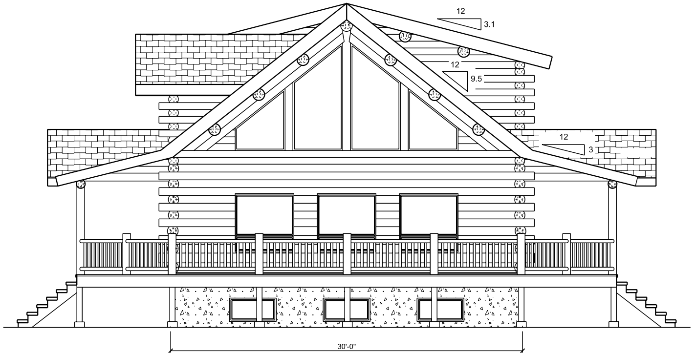
FRONT ELEVATION
