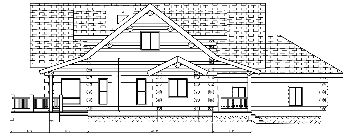
LEFT ELEVATION
