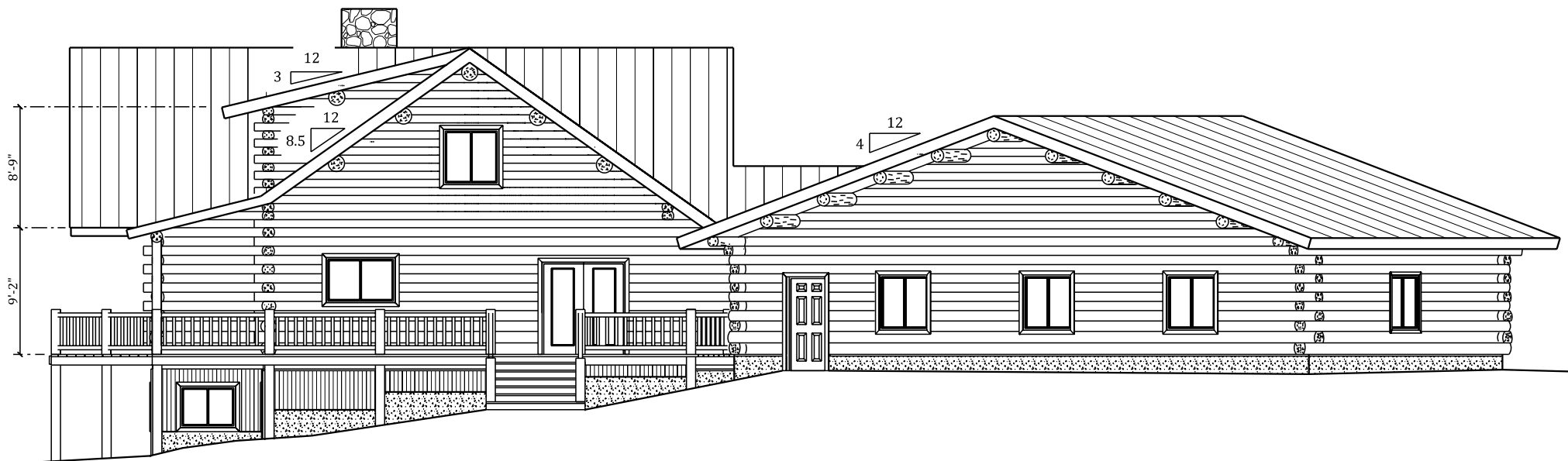
LEFT ELEVATION
