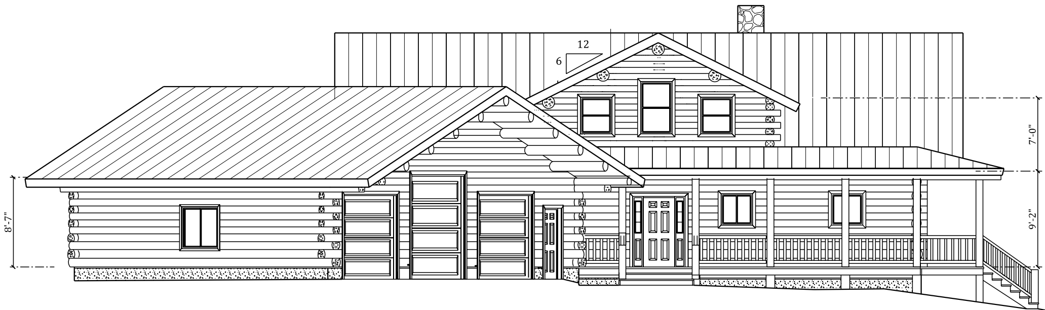
REAR ELEVATION
