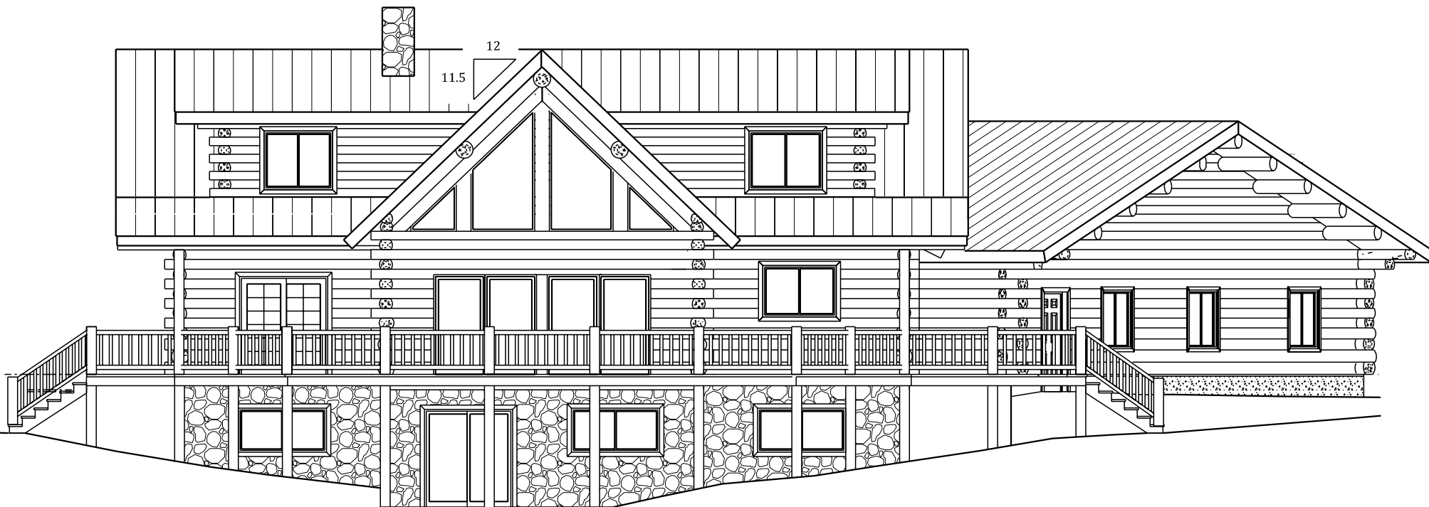
FRONT ELEVATION
