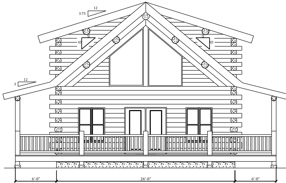
FRONT ELEVATION
