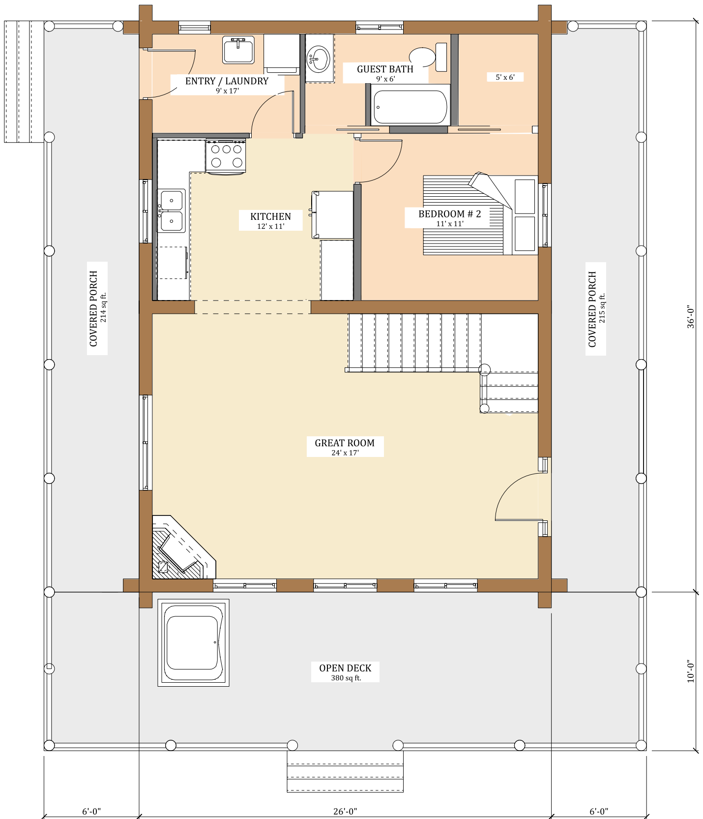
MAIN FLOOR
