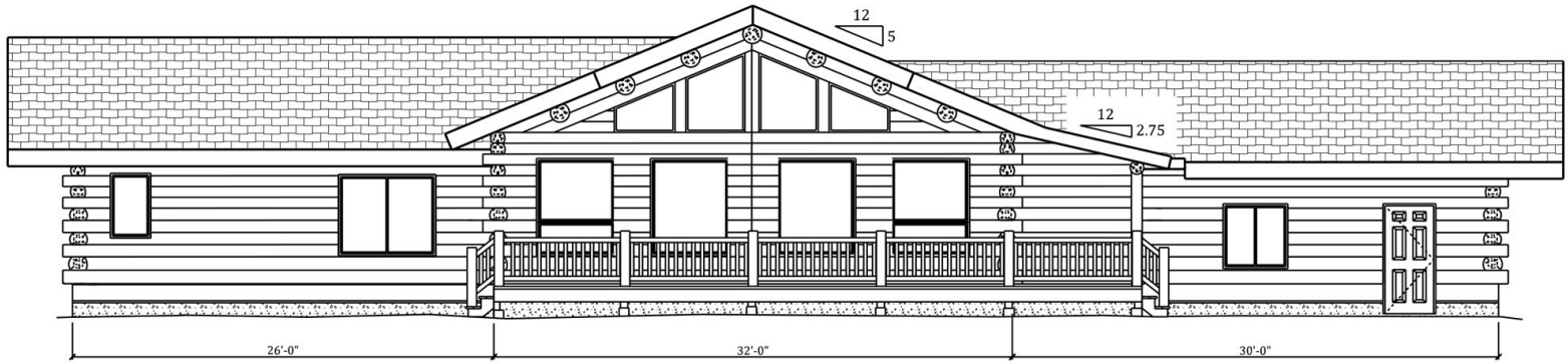
FRONT ELEVATION
