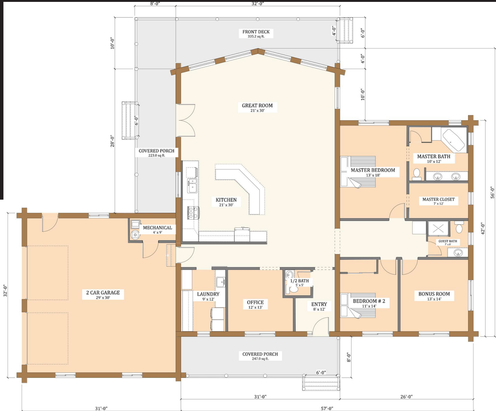
MAIN FLOOR
