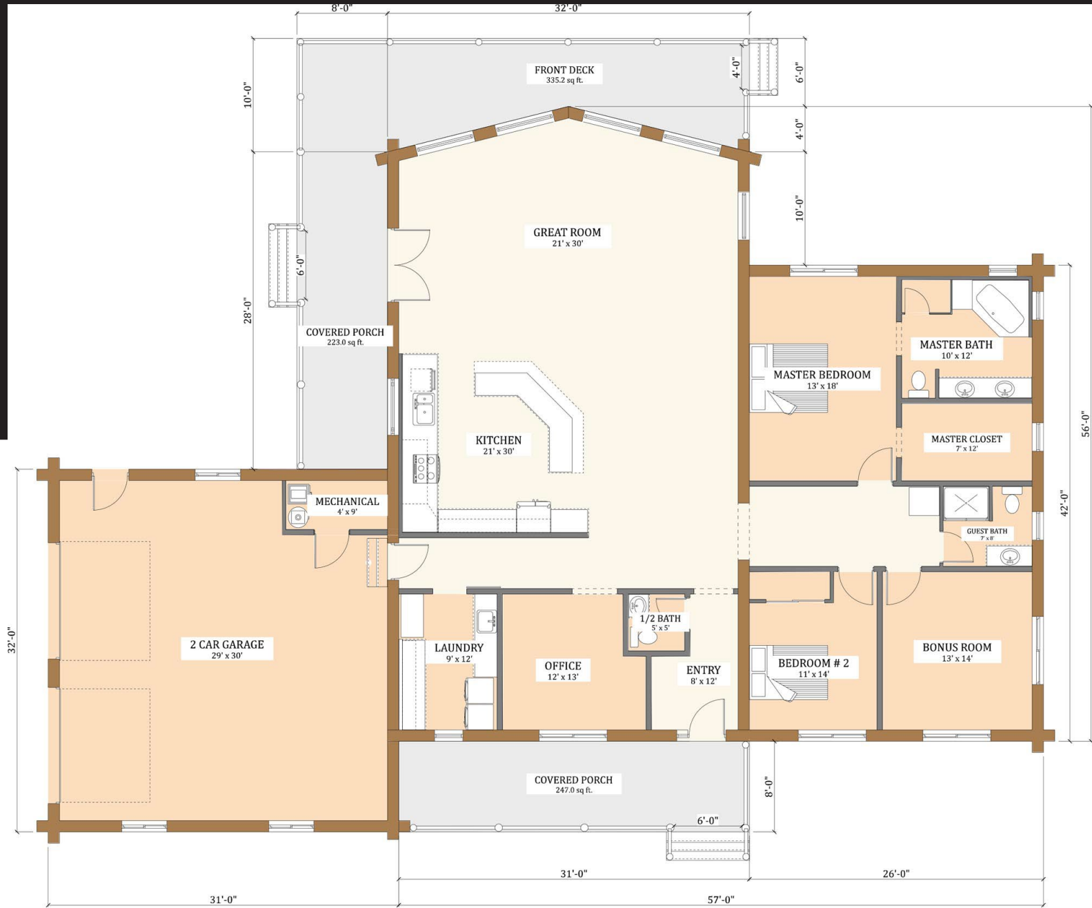
MAIN FLOOR
