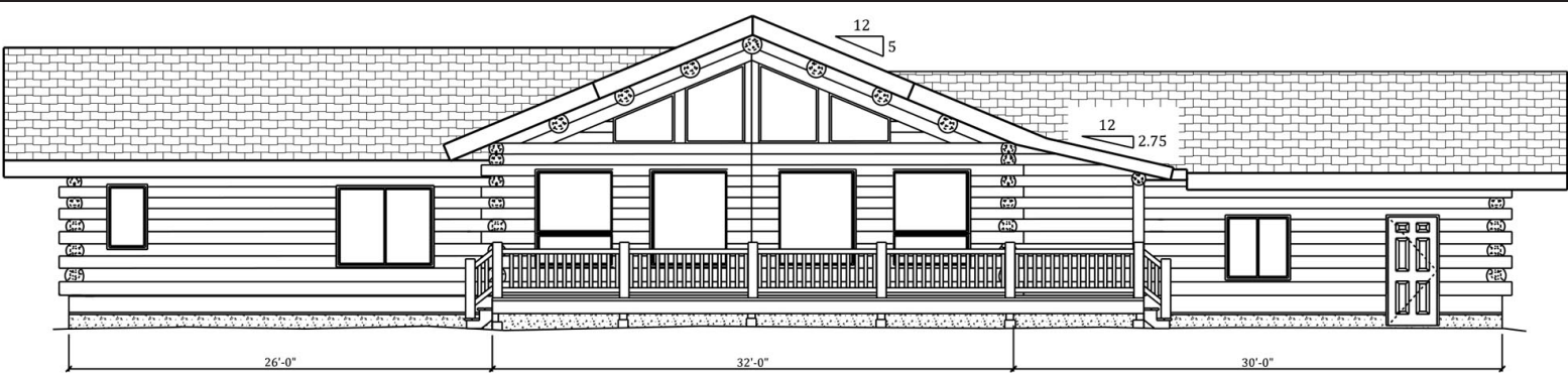
FRONT ELEVATION
