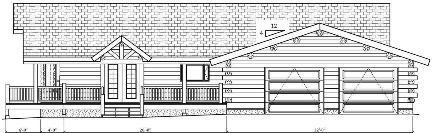
LEFT ELEVATION
