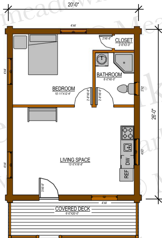
20'X26' CABIN
