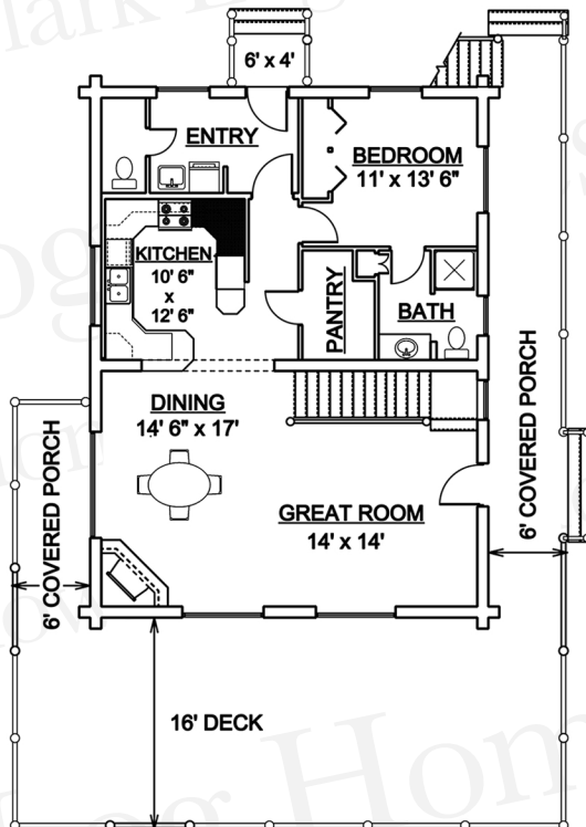
MAIN FLOOR 1200 Sq. Ft.
