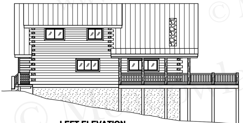
LEFT ELEVATION
