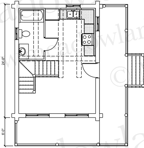
MAIN FLOOR
